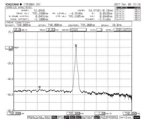
785nm Spectrum (SMSR&gt;40dB)
