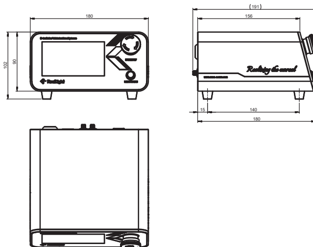
Power Supply
