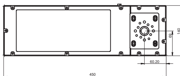
HQF-1064/532-10-6-800/400-N & HQF-1064/532-10-6-1200/600-N
