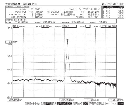
785nm Spectrum (SMSR>40dB)
