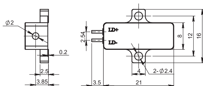
F1A Drawing
