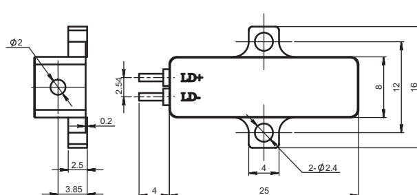
F2A Drawing
