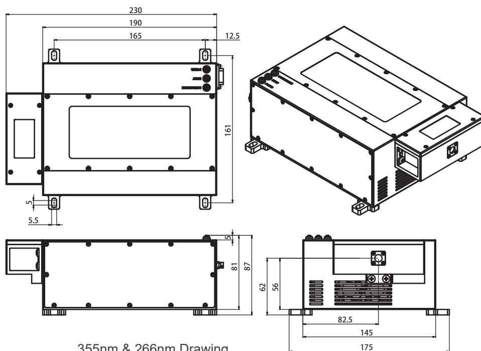
355nm & 266nm Drawing
