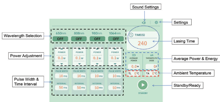
Control Screen
