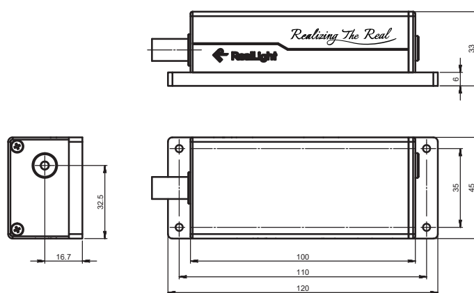
Laser Head (side laser outlet)
