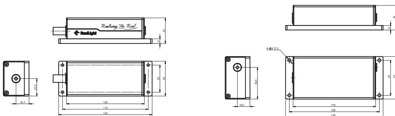
Laser Head (200 \mu J)
