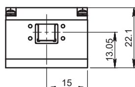
Laser Head
