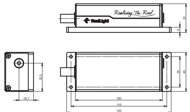
Laser Head
